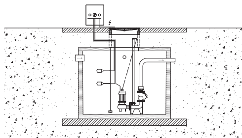
Positioning concrete pump installation type p1000
