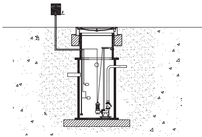
Positioning HDPE pump type PEV1000
